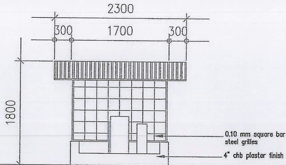
FRONT ELEVATION
