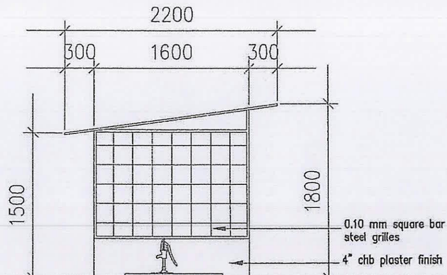
RIGHTSIDE ELEVATION
